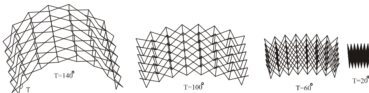
Various folding stages of a foldable double layer barrel vault
