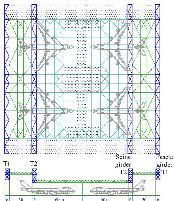
Tehran overhaul Hangar, plan: 196×200 m, span: 156 m, height: 35 m, MSA, Namvaran, SAFIRA, M Heristchian, 1998
