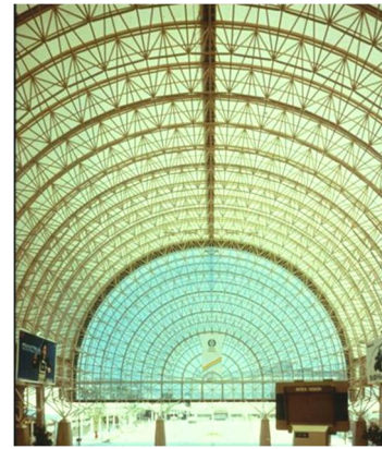
Intex Plaza exhibition hall, double layer steel barrel vault with Teflon coated fiber glass fabric for cladding and with glass gable ends, 72 m long with a span of 42 m, Osaka, Japan, 1985
