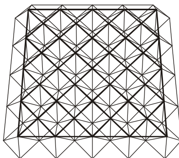
A double layer grid with mansard edges
