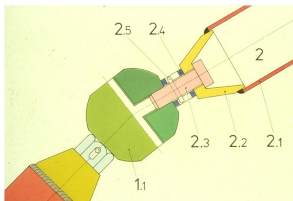
Sketch of a Mero node, showing (1.1) steel ball, (2.1) steel tube, (2.2) end cone, (2.3) high tensile bolt, (2.4) sleeve with windows and (2.5) steel pin to connect the bolt to the sleeve
