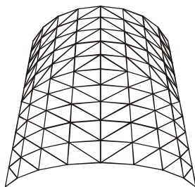
Barrel vault with a binate pattern and additional diagonal elements
