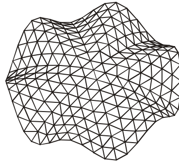
Scollap dome with sinusoidal curviance
