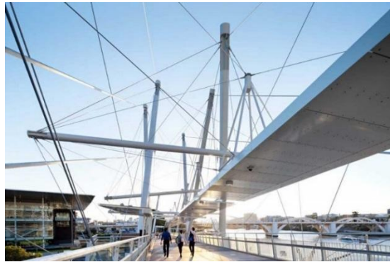
A tensegrity bridge, an example of a cable-strut system, Kurilpa tensegrity bridge, Brisbane, Australia
