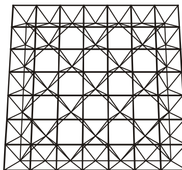
Double layer grid with a binate on larger lamella pattern
