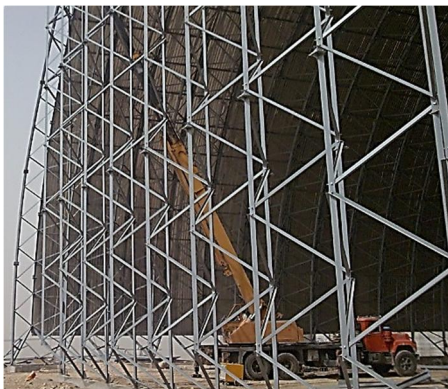
Sufian cement factory material store, span: 67 m, length: 201 m, Iran, Tabriz, Sufian, 2006, M Heristchian, Porsaz Co
