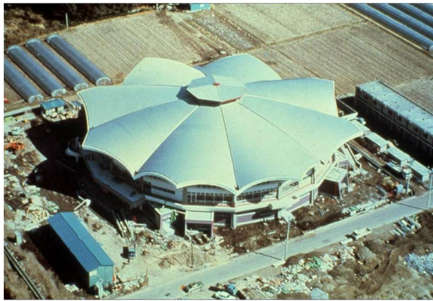
Moka City sports centre, scallop dome with eight sectors, 74 m diameter, Tochigi, Japan, 1976, Tomoe Corp
