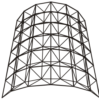
Double layer barrel vault with a binate on binate pattern
