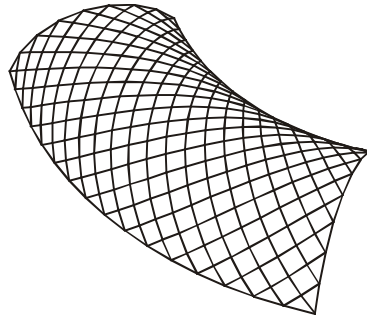
An example of sidebent annular barrel vault with lamella pattern
