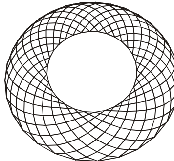
Ring barrel vault with lamella pattern
