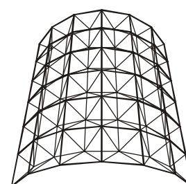
Double layer barrel vault with binate on binate pattern
