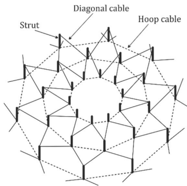
General form of arrangement of hoops, struts and diagonals in a suspen-dome
