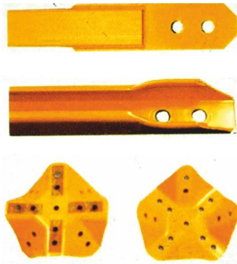
An example of a plate node, the KE system
