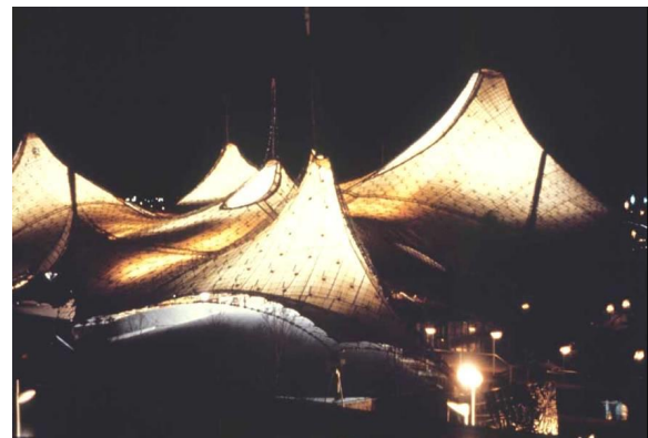
Night view of the West German Pavilion cable structure, Montreal Expo 67, Frei Otto
