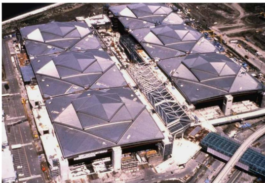
Aerial view of a complex of six stepping steel double layer grids, 90 m x 90 m each, Tokyo, Japan, 1994, Tomoe Corp
